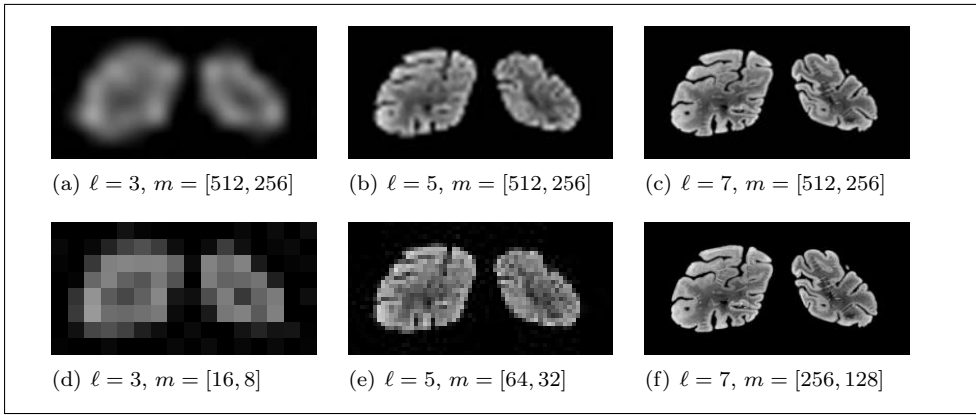
Figure 6.15: Multilevel representation of the data T^\ell (a-c) and the functions T^\ell(xc^\ell) , \ell = 3, 5, 7 (d-f).
