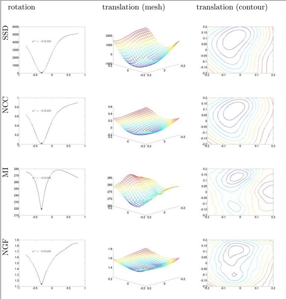
Figure 7.2: Distance measures for the monomodal images shown in Figure 7.1. Left column: distance versus rotations around the domain center, middle/right columns: mesh/contour plots of distance versus translation.
