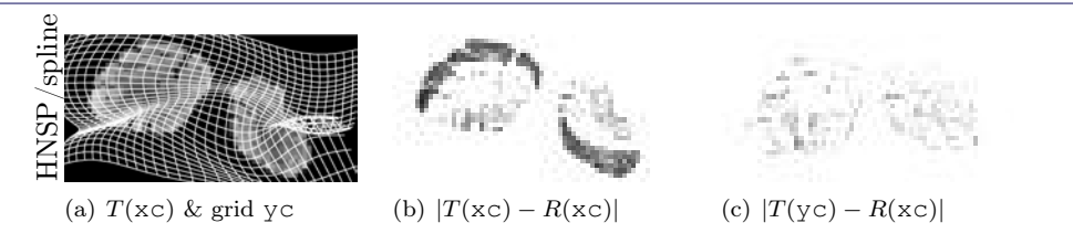
Figure 6.13: PIR results for SSD and spline transformation, m = [32, 16] and p = [4, 5] ; yc = y(wc, xc) .
