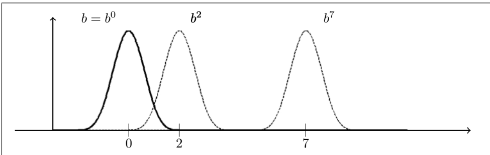
Figure 3.6: “Mother” spline b = b^0 (solid) and basis functions b^2 and b^7 .
