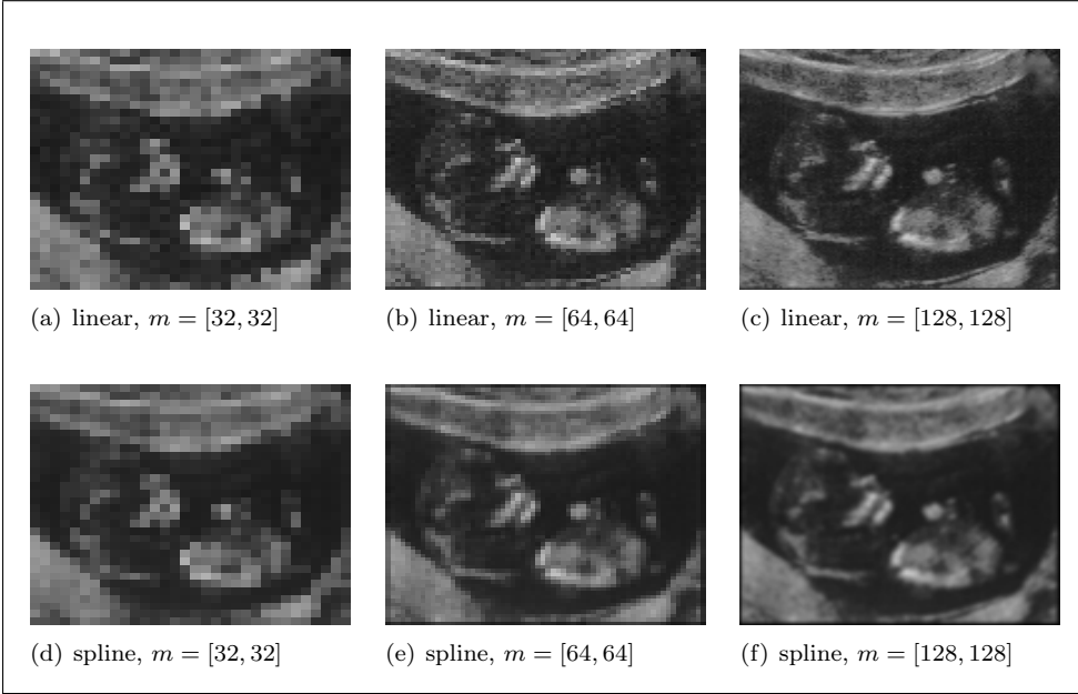
Figure 3.14: Interpolation on duty: linear and spline interpolation on a cell-centered grid of dimension m ; see Example 3.20.
