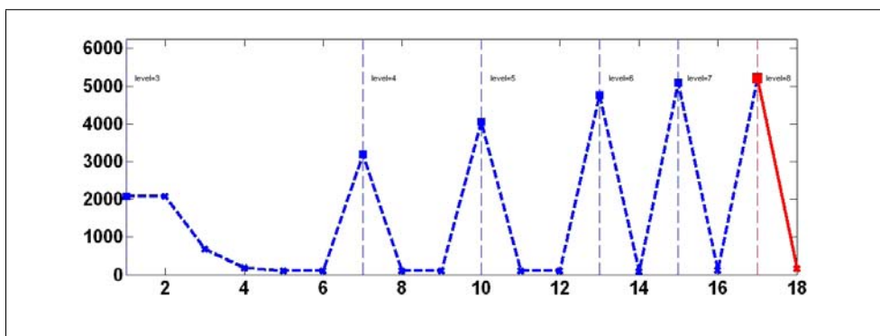
Figure 6.18: Iteration history for MLPIR with SSD and affine2D, J(w^k) versus k : vertical dashed lines separate different levels; reference values on the \ell th level are shown as squares; iterations as crosses; on finest level ( \ell = 8 ) only a comparison step is needed.
