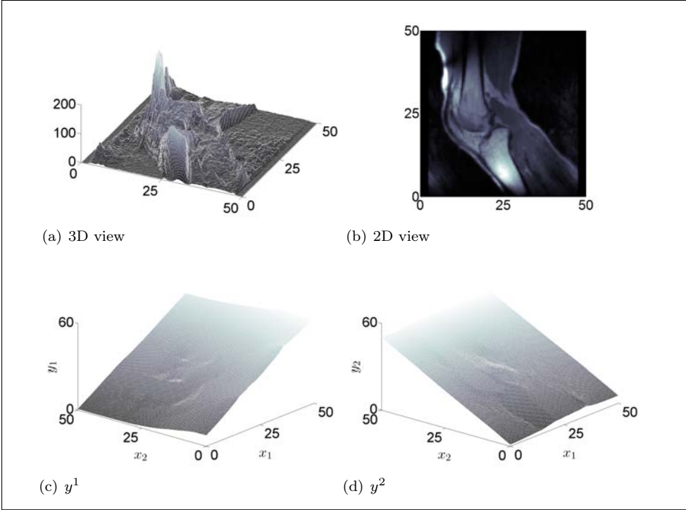
Figure 2.1: Visualizations of an image and a transformation y = (y^1(x^1, x^2), y^2(x^1, x^2)) .
