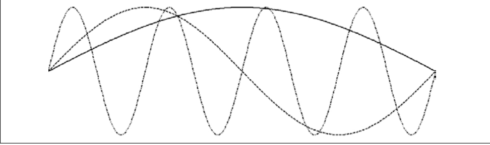
Figure 3.11: Oscillations: j th column of V ( m = 8 ), j = 1 (solid line), j = 2 (dashed line), and j = 8 (dashed-dotted line).
