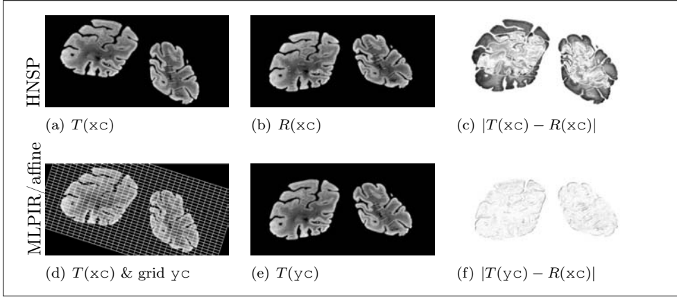
Figure 6.19: MLPIR results for distance = SSD, trafo = affine2D, and m = [512, 256] ; yc = \text{trafo}(wc, xc) , wc \approx [0.959, 0.305, -0.122, -0.310, 0.966, 0.339] , reduction \approx 0.0314 .
