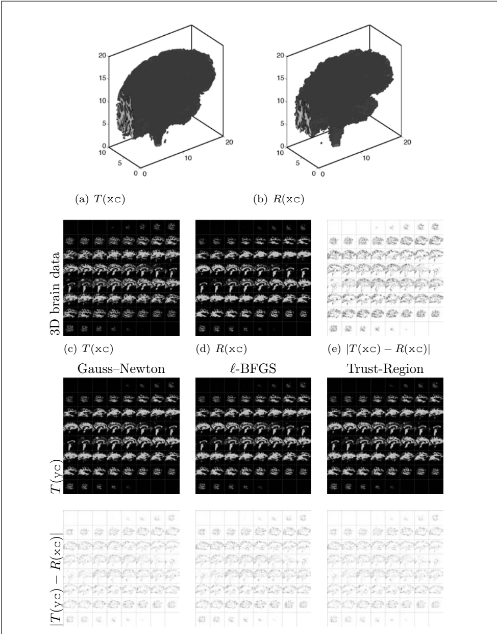
Figure 9.11: MLIR results for 3D brain data (cf. Example 9.10) using the SSD distance combined with a curvature regularizer; 3D (top row) and 2D (second row) visualizations of the template and reference images. Transformed template (third row) and differences to the reference image (bottom row) are shown for optimization results obtained with Gauss-Newton (left), \ell -BFGS (middle), and trust-region (right); see Example 9.8 for details.
