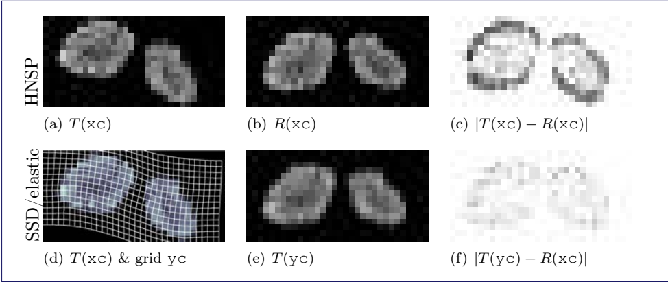
Figure 9.1: NPIR results for HNSP data; cf. Example 2.8: splineInter2D , SSD , mbElastic/staggered , [\alpha, \mu, \lambda] = [10000, 1, 0] , \Omega = (0, 2) \times (0, 1) , level = 4 , m = [32, 16] , \#iter = 16 , reduction = 25.45%.
