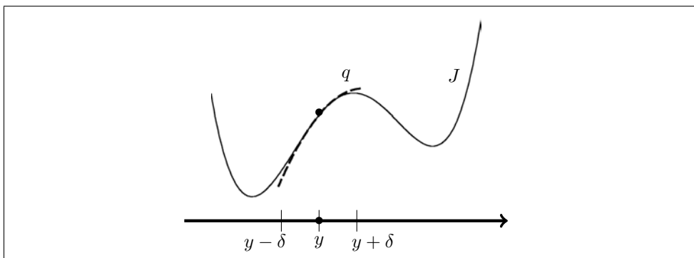
Figure 9.9: Objective function J , quadratic model q , and trust-region \{z : |z - y| \leq \delta\} .
