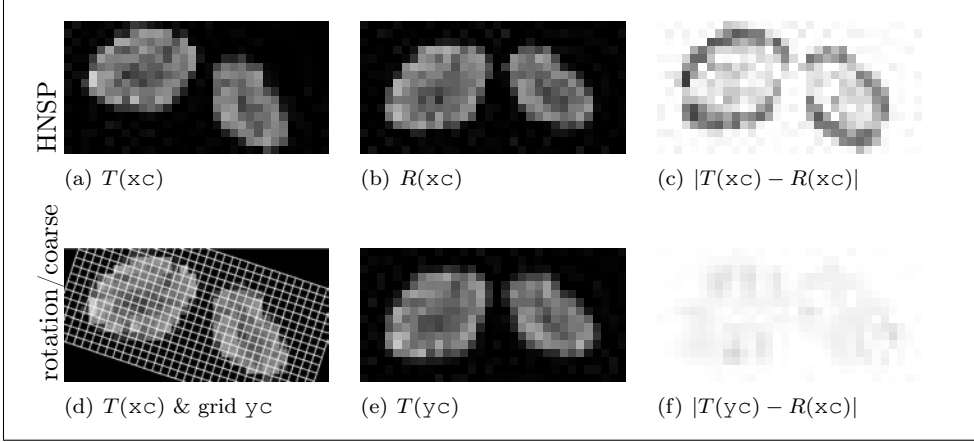
Figure 6.7: PIR results for distance = SSD, trafo = rotation2D, and m = [32, 16] ; yc = y(wc, xc) , wc = w^7 \approx -0.3229 , reduction \approx 8.4\% .
