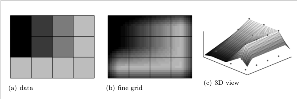
Figure 3.5: Linear interpolation of the data of Example 3.7 (a particular colormap has been used for (a) and (b)).
