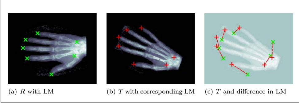
Figure 5.1: Reference and template with corresponding landmarks r_j = [r_j^1, r_j^2] (green \times ) and t_j = [t_j^1, t_j^2] (red + ), and landmark errors (red dashes).
