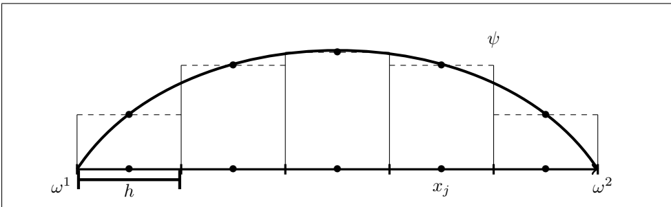
Figure 6.1: Midpoint quadrature rule in one dimension.
