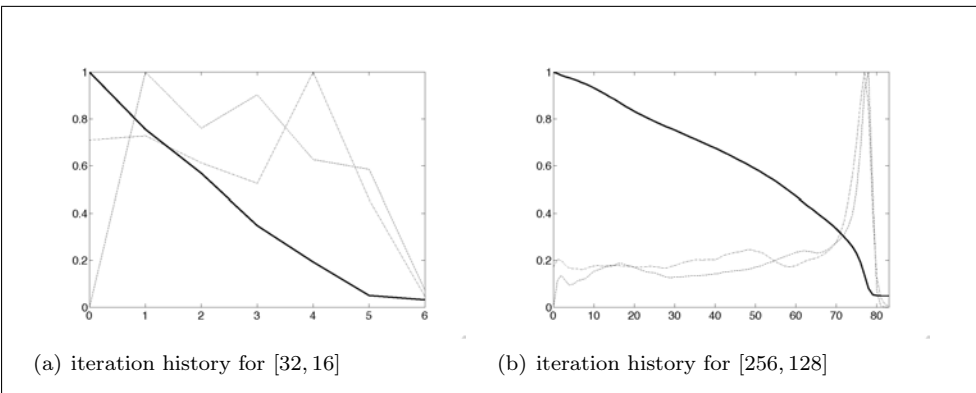
Figure 6.12: Iteration history for PIR with SSD and rigid2D: coarse (left) and fine (right) discretization; J(w^k) (solid line), \|w^k - w^{k-1}\| (dashed line), and \|d_w J(w^k)\| (dashed dotted line); all numbers are relative.
