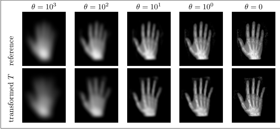
Figure 9.3: Multiscale image registration results for hand data; cf. Example 2.7; scale \theta = 10^3, 10^2, 10, 1, 0 ; visualization of reference image on different scales (top row) and transformed template (bottom row): splineInter2D , regularized by moments and \theta = 10^3, 10^2, 10, 1, 0 , SSD , mbElastic/staggered , [\alpha, \mu, \lambda] = [10000, 1, 0] , \Omega = (0, 20) \times (0, 25) , level = 7, m = [128, 128] , #iter = [6, 2, 2, 4, 2, 2], reduction \approx 2.36\% .
