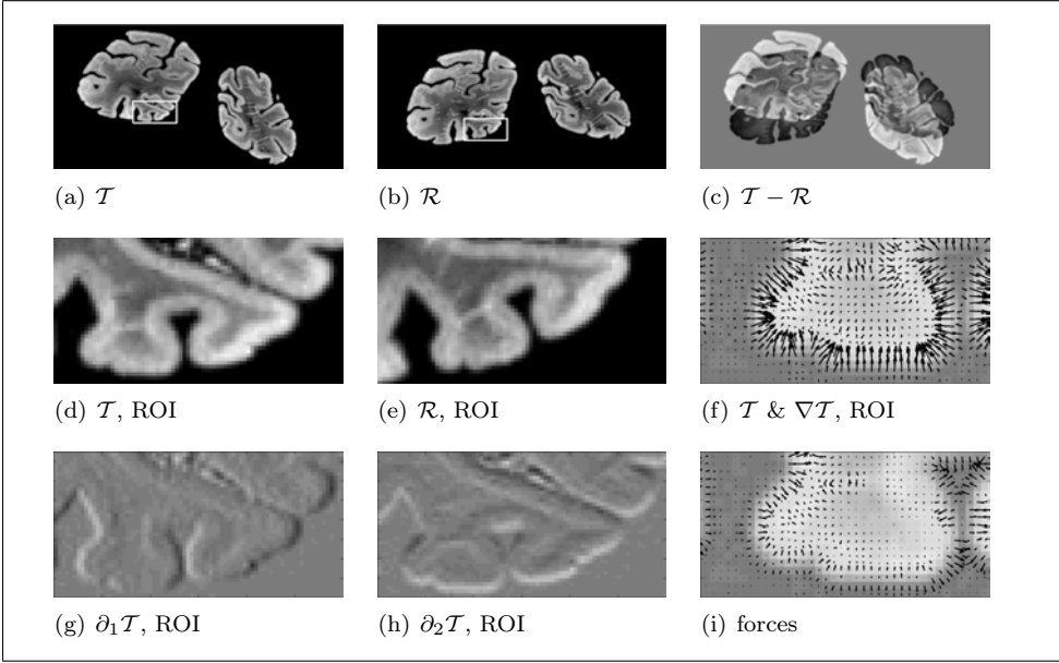
Figure 7.1: Forces of the SSD: (a) template \mathcal{T} with a region of interest (ROI); (b) reference \mathcal{R} with ROI; (c) difference \mathcal{T} - \mathcal{R} ; ROIs of (d) \mathcal{T} , (e) \mathcal{R} , (f) \nabla \mathcal{T} , (g) \partial_1 \mathcal{T} , (h) \partial_2 \mathcal{T} ; and the (i) force field.
