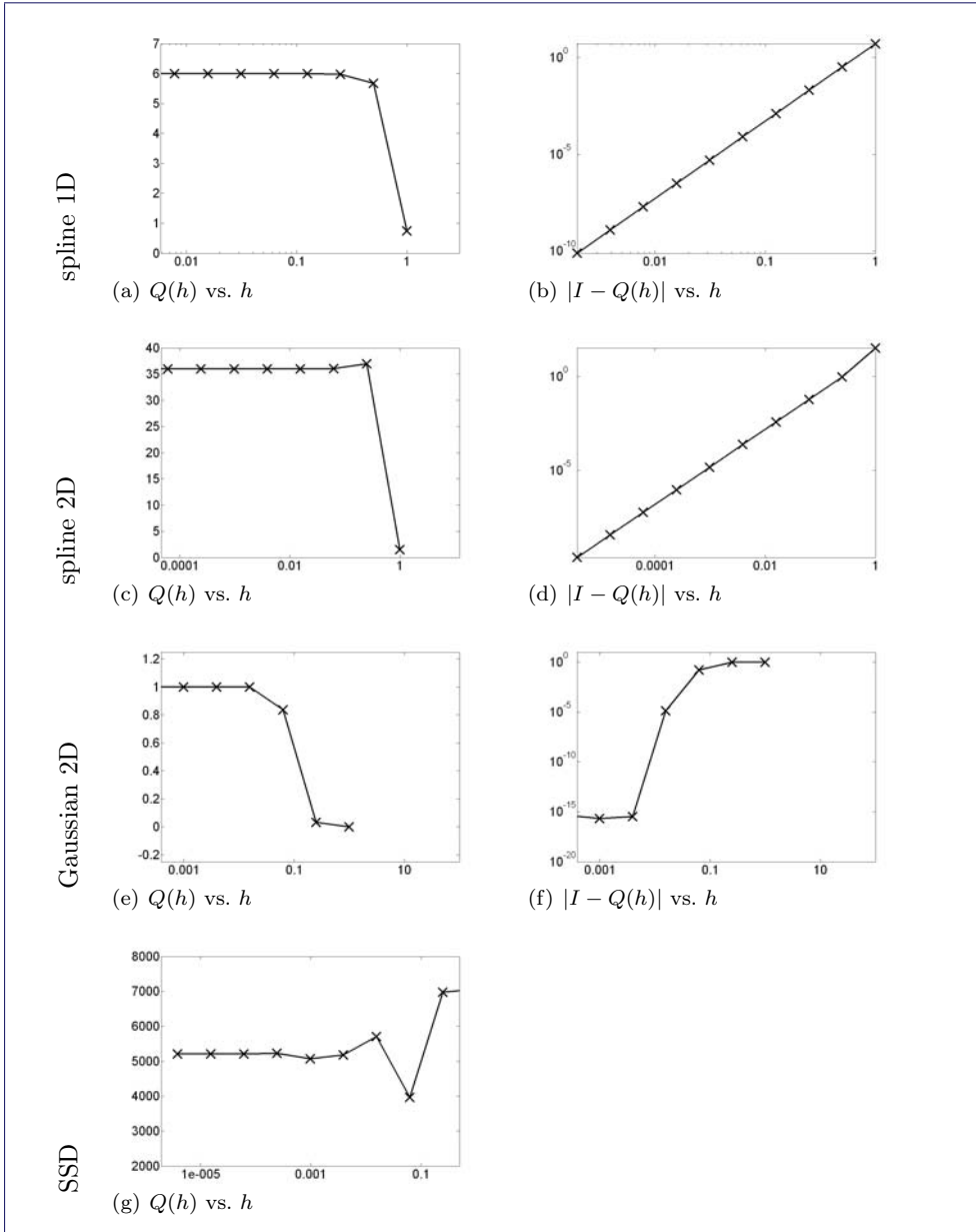
Figure 6.2: Quadrature on duty for various functions \psi .
