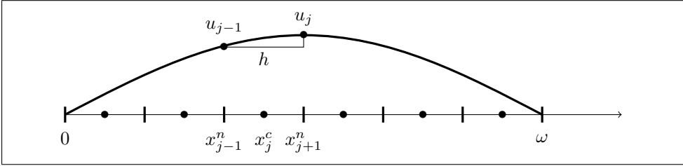
Figure 8.2: Cell-centered finite difference approximation of a derivative.
