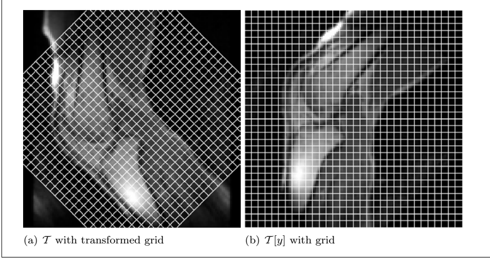
Figure 2.2: Transforming images.
