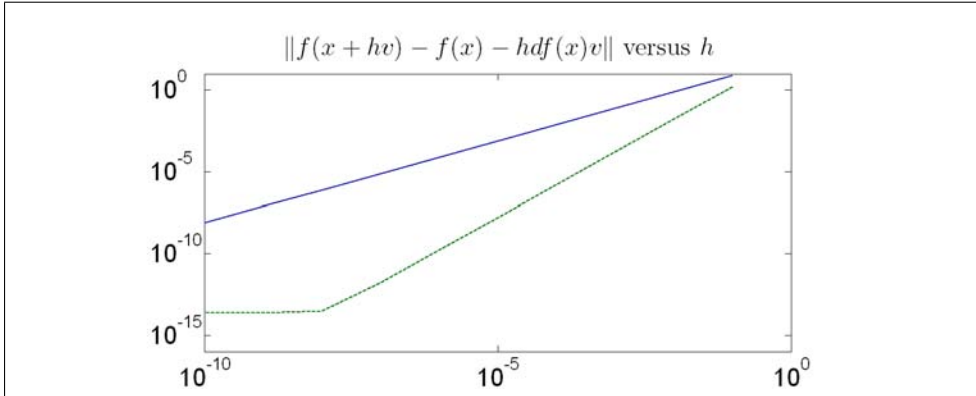
Figure 3.9: A typical result of checkDerivative : linear decay (solid line) for \|f(y + hv) - f(y)\| and quadratic decay (dashed line) for \|f(y + hv) - f(y) - hdf(y)\| up to machine precision shown on a logarithmic scale.
