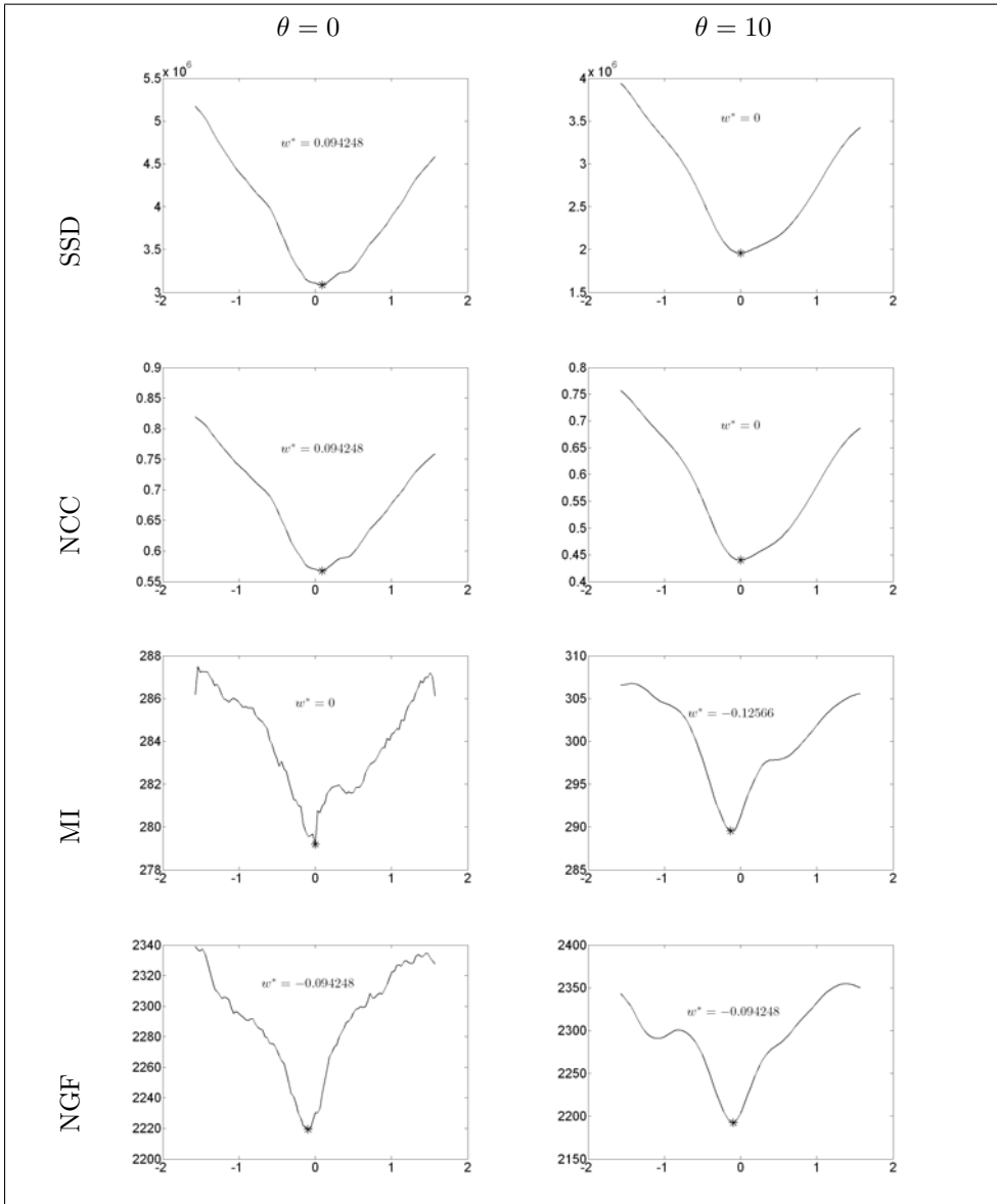
Figure 7.9: Distance measures versus rotation angle for PET/CT images; see Example 7.8. Left/right columns: using scale parameters \theta = 0, 10 .
