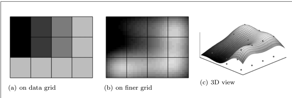
Figure 3.8: Spline interpolation of the data of Example 3.7 (a particular colormap has been used in (a) and (b)).
