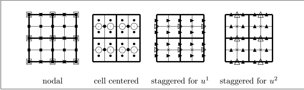
Figure 9.4: Prolongation of 2D grids.
