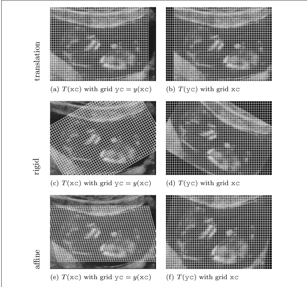
Figure 4.1: Translation of a US image, rigid, and affine linear transformations.
