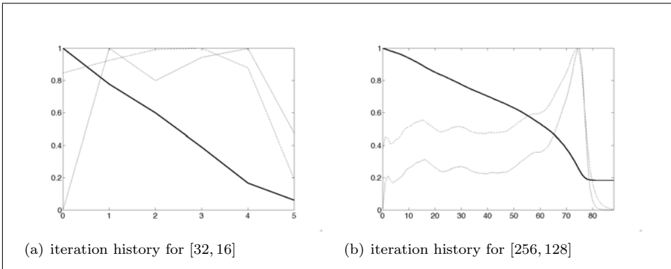
Figure 6.9: Iteration history for PIR with SSD and rotation2D: coarse (left) and fine (right) discretization; J(w^k) (solid line), \|w^k - w^{k-1}\| (dashed line), and \|d_w J(w^k)\| (dashed dotted line); all numbers are relative.
