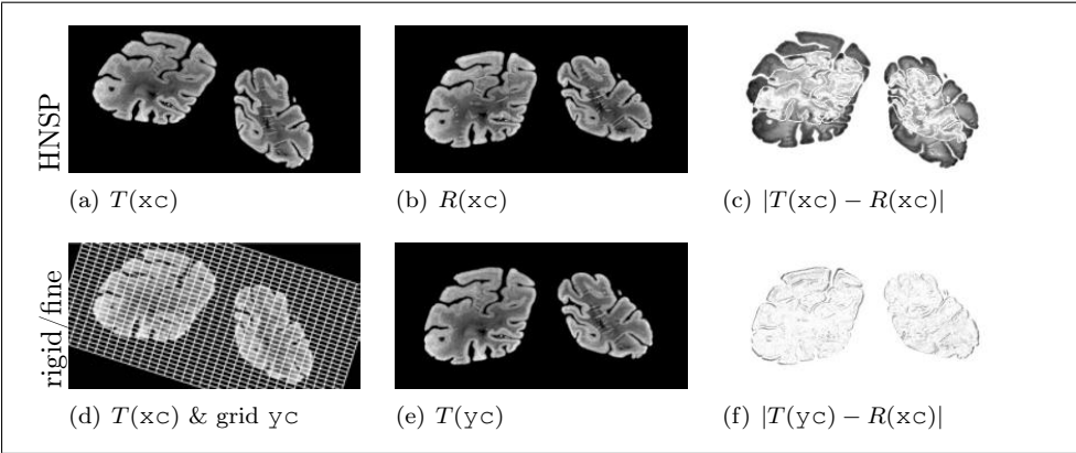
Figure 6.11: PIR results for distance=SSD, trafo=rigid2D, and m = [256, 128] ; wc = w^{72} \approx [-0.3130, -0.1156, 0.3444] , reduction \approx 4.4\% .
