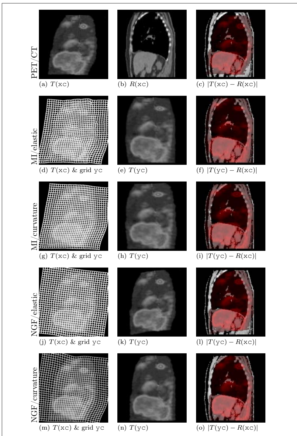
Figure 9.8: MLIR results for PET/CT data (cf. Example 2.10) using MI and NGF distances combined with elastic and curvature regularization and \ell -BFGS optimizer; see Example 9.8 for details.
