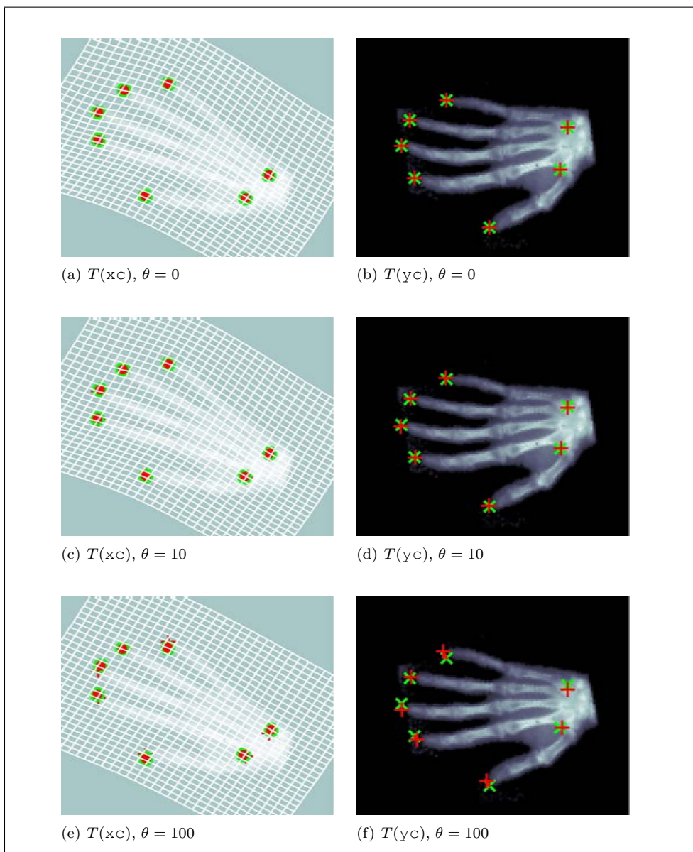
Figure 5.3: Thin-plate-spline registration with various \theta 's.
