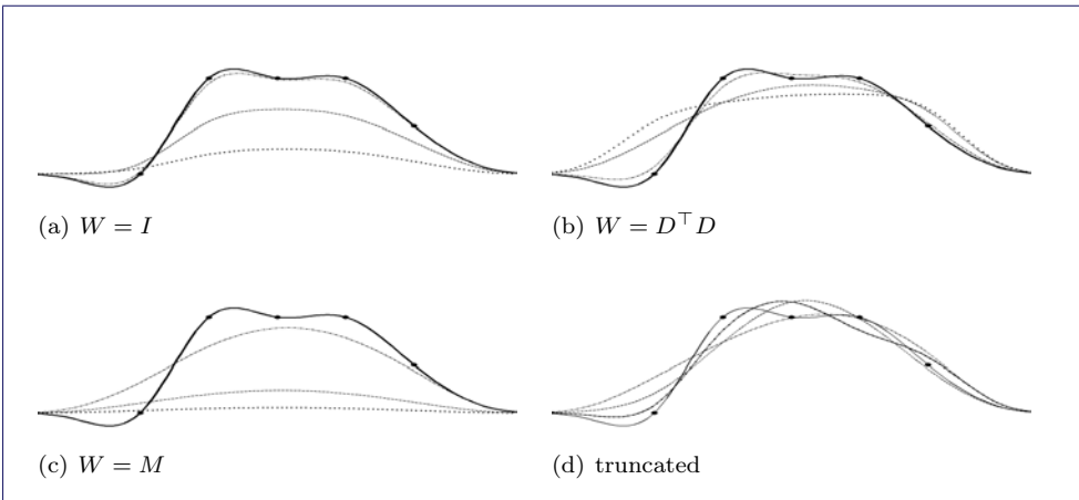
Figure 3.10: Spline approximations with different regularization and varying \theta 's, \theta = 0 (thick solid line), \theta = 1 (dashed line), \theta = 10 (dashed-dotted line), and \theta = 100 (dotted line), see Example 3.13. (d) shows results for the truncated regularization; see Example 3.14.
