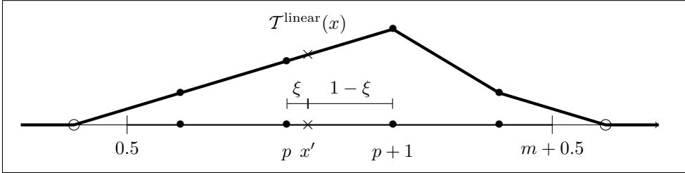
Figure 3.4: Linear interpolation in one dimension.
