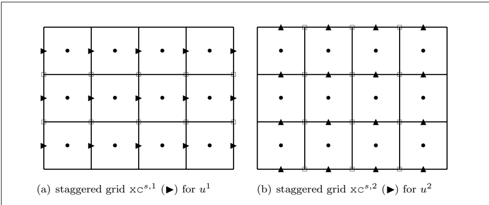
Figure 8.3: Grids for d = 2 : cell-centered x_{c^c} (●), nodal x_{c^n} (□), and staggered grids x_{c^{s,1}} (►) and x_{c^{s,2}} (▲).
