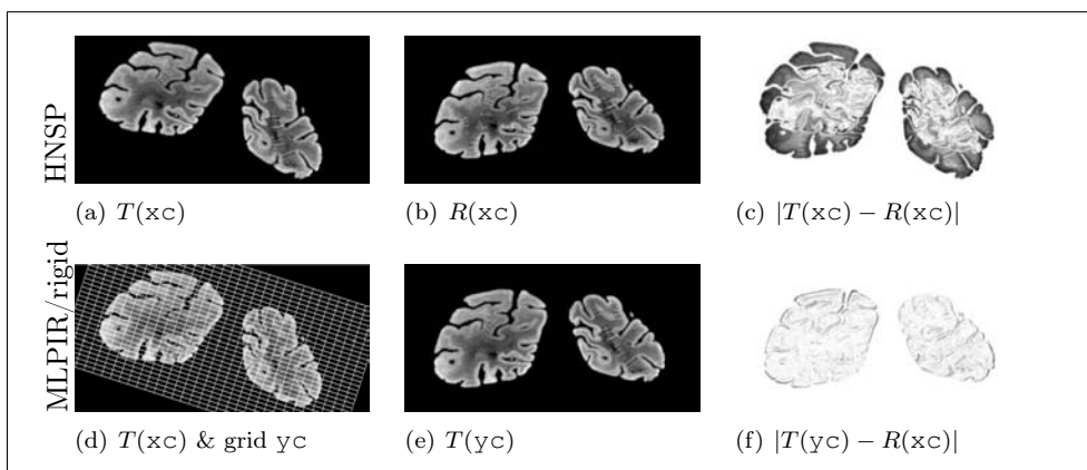
Figure 6.17: MLPIR results for distance = SSD, trafo = rigid2D, and m = [512, 256] ; yc = \text{trafo}(wc, xc) , wc \approx [-0.3128, -0.1153, 0.3440] , reduction \approx 5.8\% .
