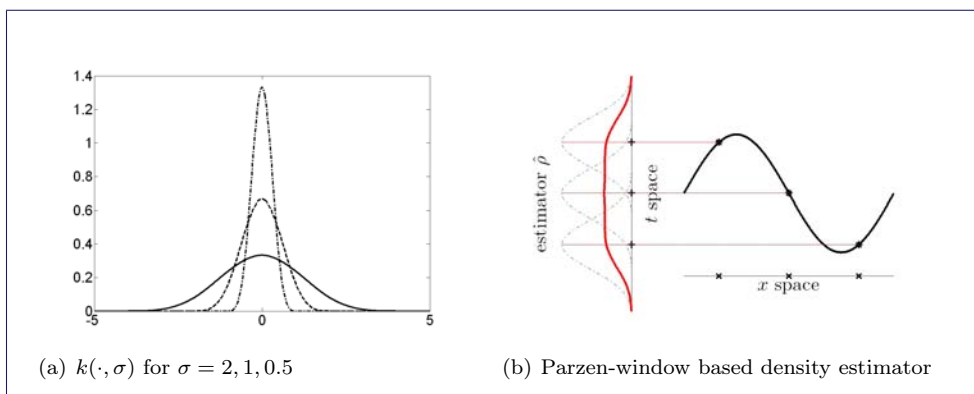
Figure 7.6: (a) Spline-based Parzen-window kernel k(\cdot, \sigma) for \sigma = 2, 1, 0.5 ; (b) Parzen-window estimator based on three samples.
