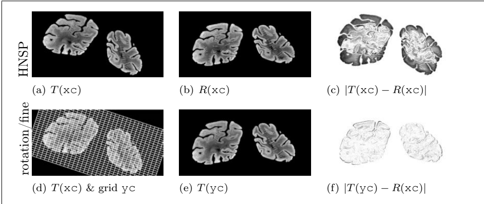
Figure 6.8: PIR results for distance = SSD, trafo = rotation2D, and m = [256, 128] ; wc = w^{81} \approx -0.3202 , reduction \approx 18.5\% .
