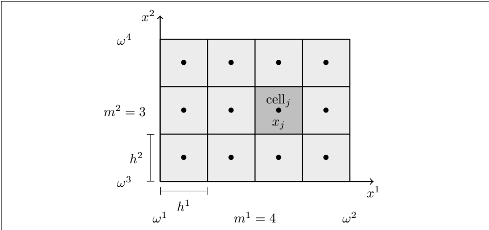
Figure 3.2: Discretization of a 2D domain \Omega = (\omega^1, \omega^2) \times (\omega^3, \omega^4) \subset \mathbb{R}^2 .
