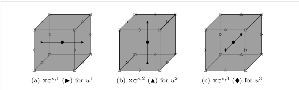
Figure 8.4: Grids for d = 3 on a cell: cell-centered x_C^c (●), nodal x_C^n (□), and staggered grids x_C^{s,1} (►), x_C^{s,2} (▲), and x_C^{s,3} (◆).
