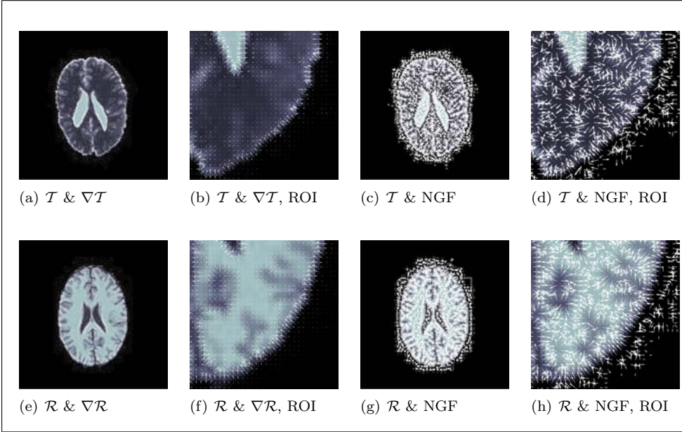
Figure 7.8: Normalized Gradient Fields (NGF) for T1/T2 weighted MRIs; cf. Example 2.9.
