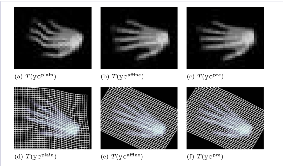
Figure 9.2: NPIR results for hand data; cf. Example 2.7: plain NPIR (left), affine linear (middle), and combined approaches (right); the configuration for the plain approach: splineInter2D , SSD , mbElastic/staggered , [\alpha, \mu, \lambda] = [10000, 1, 0] , \Omega = (0, 20) \times (0, 25) , level = 5 , m = [32, 32] , \#iter = 12 , reduction \approx 47.31\% .
