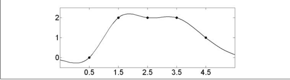
Figure 3.7: Spline interpolation in one dimension; see Example 3.8.
