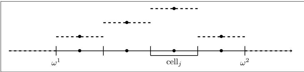
Figure 3.3: Next neighbor interpolation in one dimension (dashed line).
