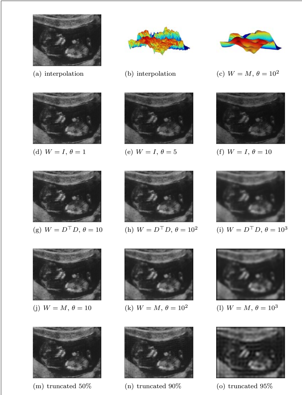
Figure 3.12: Spline approximations in two dimensions with different regularization W and varying \theta 's; (b) and (c) show 3D views of a detail in the image; image from Example 2.6.
