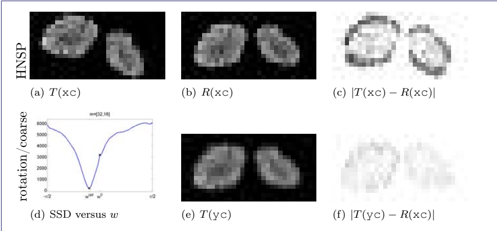
Figure 6.3: SSD versus rotations for m = [32, 16] ; y_C = y(w_C, x_C) .
