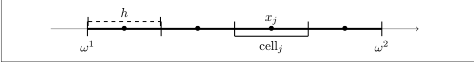
Figure 3.1: Discretization of a 1D domain \Omega = (\omega^1, \omega^2) \subset \mathbb{R} .
