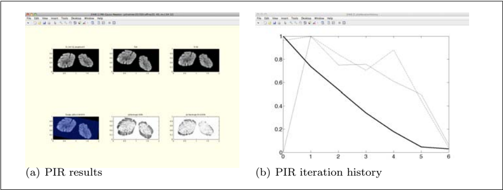
Figure 6.6: Plots from PIR.
